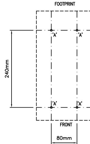
DRILLING DETAIL
