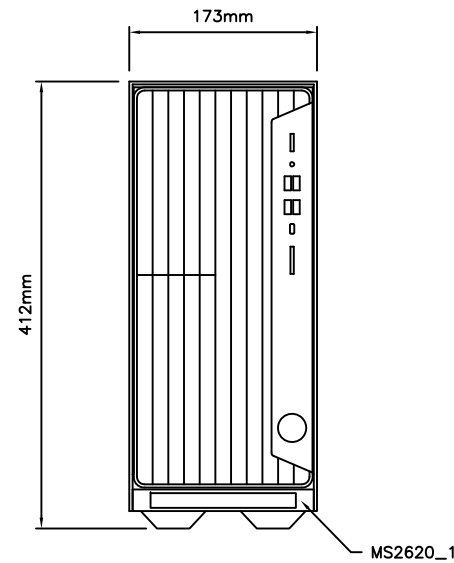
FRONT ELEVATION
